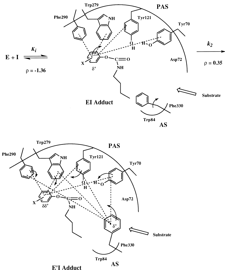
Figure 4. The proposed mechanism for the inhibition of AChE by carbamates 1–9 at the PAS of the enzyme. Numbers refer to residue positions in Torpedo californica AChE. 3
