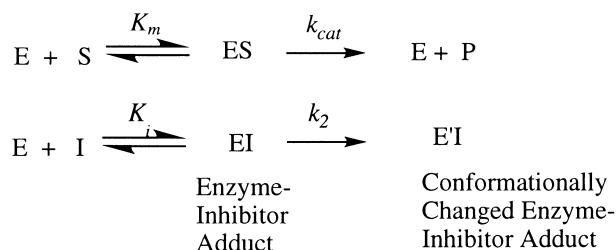
Scheme 1. Kinetic scheme for irreversible inhibition of AChE in the presence of substrate.
