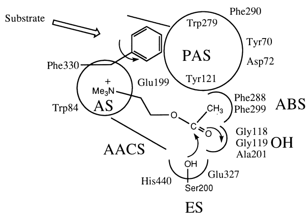
Figure 1. The active site and the PAS of AChE. Numbers refer to residue positions in Torpedo californica AChE. 3
