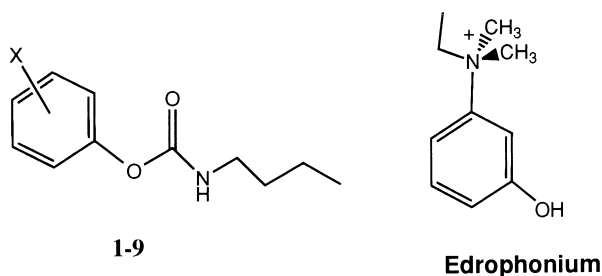
Figure 2. Chemical structures of carbamates 1–9 and edrophonium.
