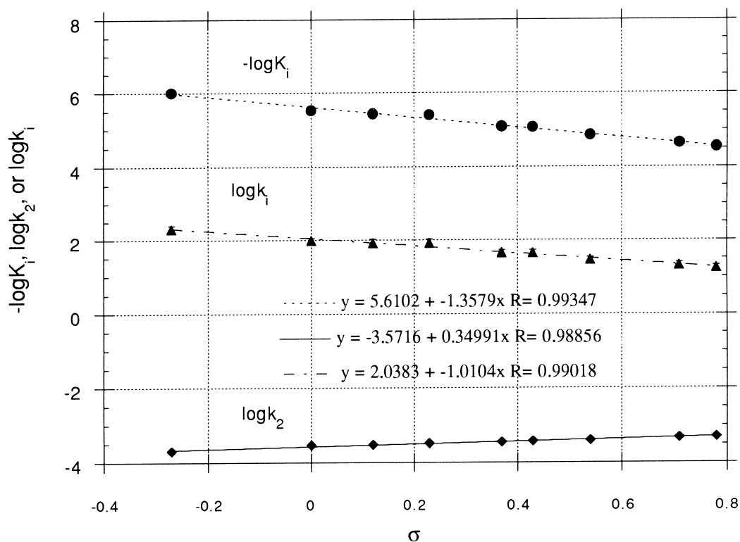
Figure 3. Plot of -\log K_i , \log k_2 , and \log k_i for the inhibition of AChE by carbamates 1–9 against \sigma .
